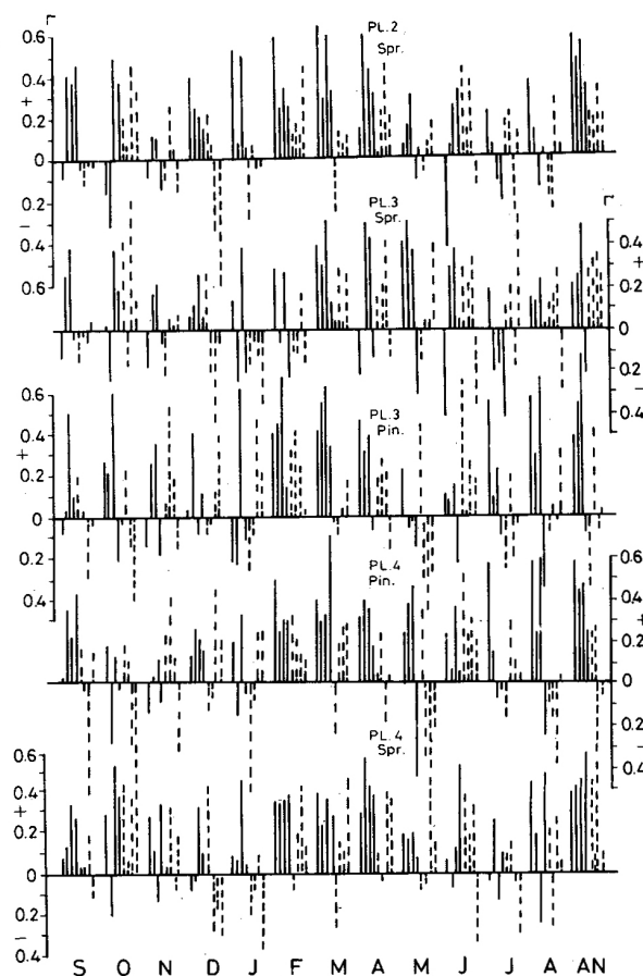
Text-figure 1 —Pine and Spruce radial growth correlation with average monthly and annual weather data. From left to right, the coefficients for the first, second, third and fourth periods ——— with temperature ——— with precipitation.
